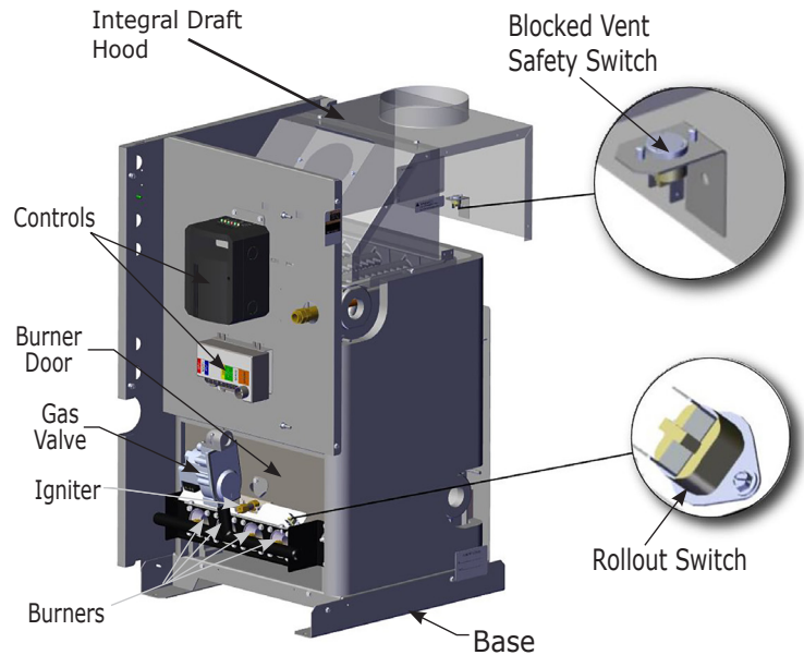
FIGURE 2 - BOILER FLUE GAS PASSAGEWAYS
